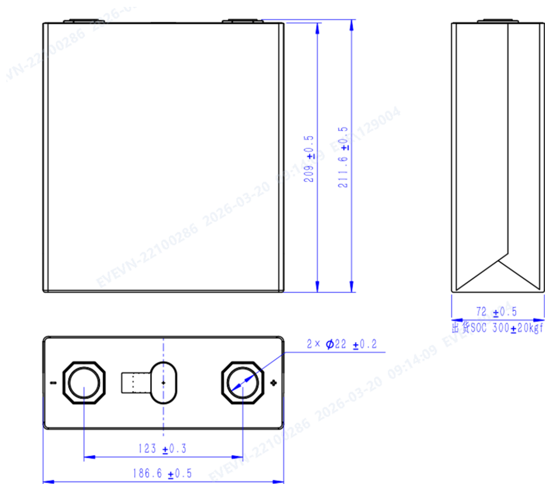
Fig. 15 Diagram of cell size and appearance
