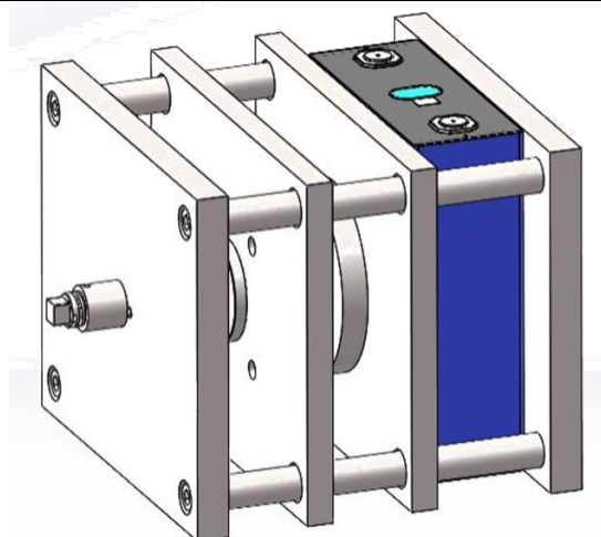
Fig. 5 Diagram of cell with swelling force clamp
