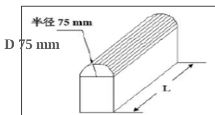
Fig. 6 Diagram of the Extrusion Device
