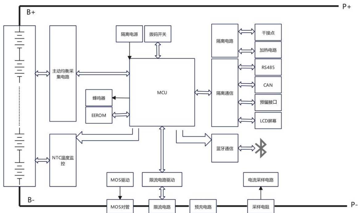
JK-PB1/2A16S-10/15/20P 结构框图
